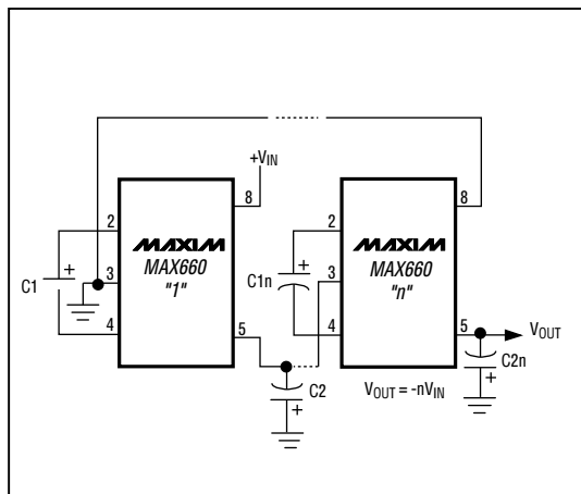
Figure 3. Cascading MAX660s to Increase Output Voltage
